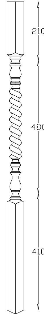
Spindle 1100mm
